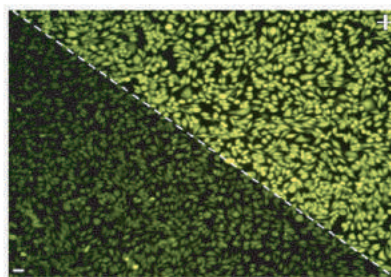
Calcium Response
