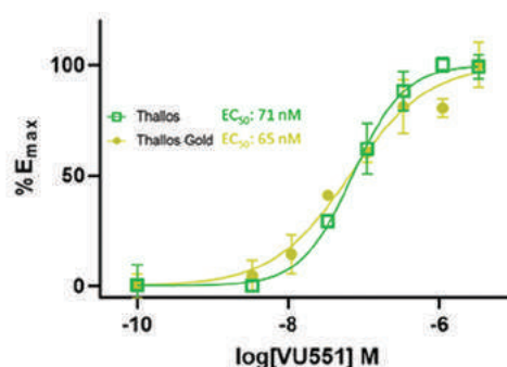
GIRK ( K_{ir} 3.1/3.2) Assay
