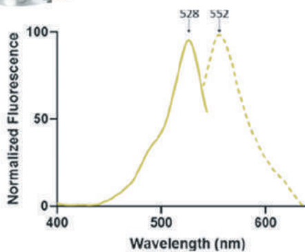
Fluorescence Spectra
